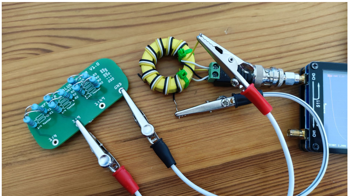
1:9 Balun
